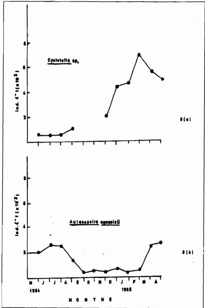
Fig. 8: Seasonal variation in the dominant Bacillariophyta; Cyclotella sp (8a) and Aulacoseira agassizii (8b) at L. Baringo during the sampling period
