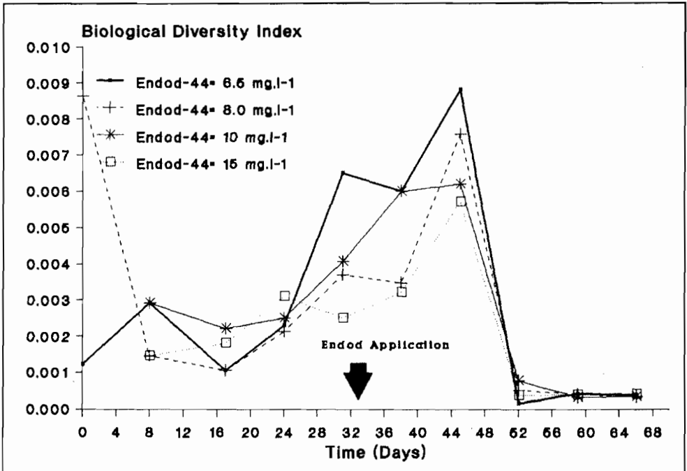
Figure 2: Variations of the diatom biological diversity index in basins
