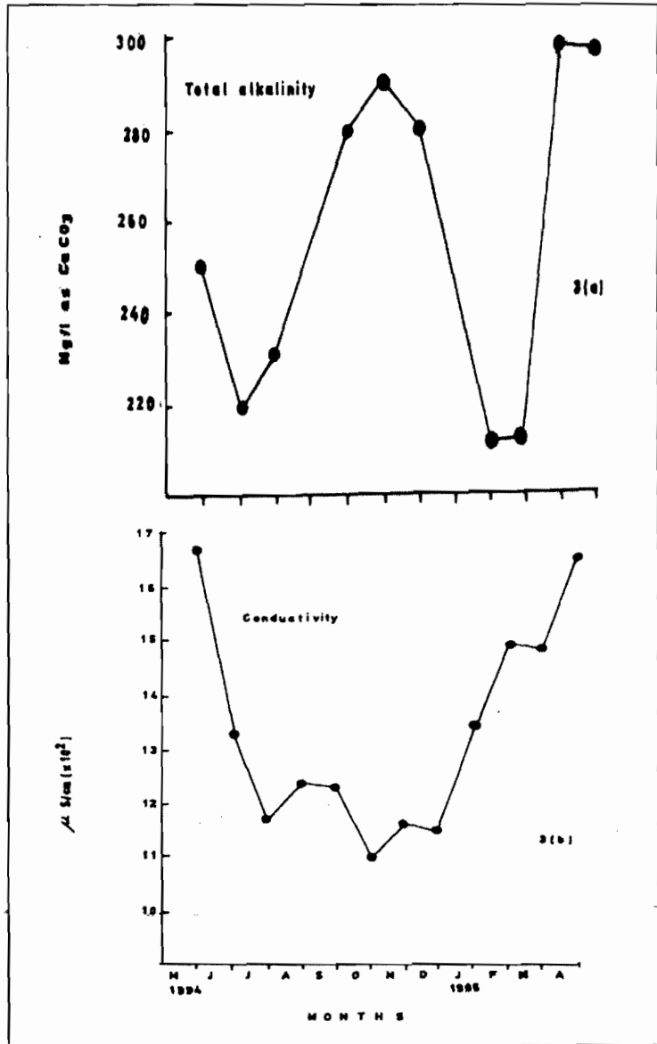
Fig 3a: Temporal variation in Total alkalinity at L. Baringo during the sampling period
