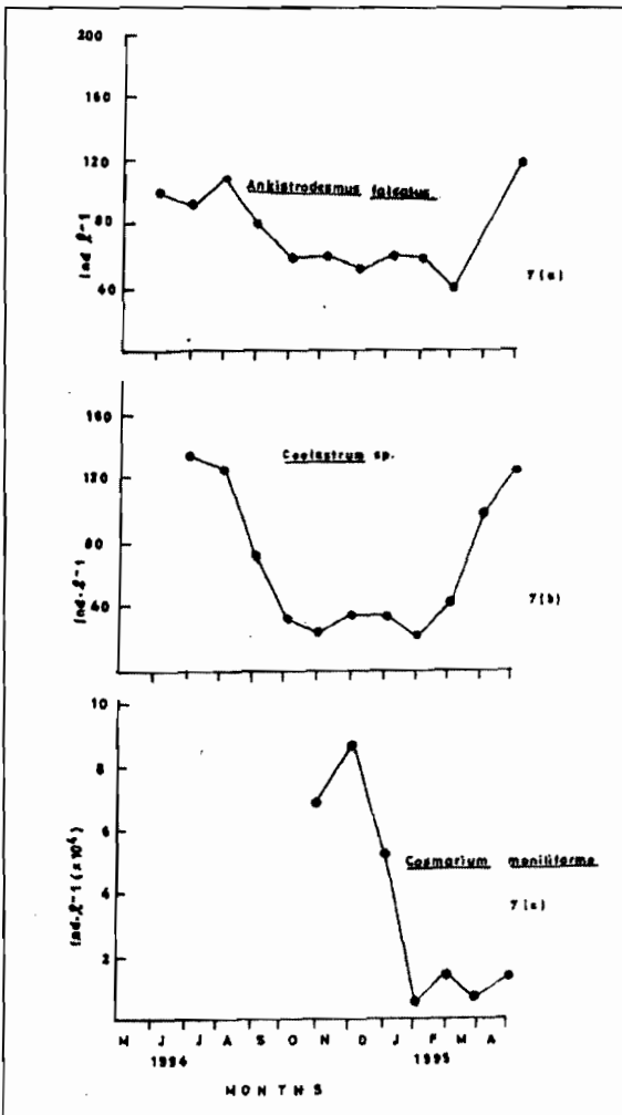
Fig. 7: Seasonal variation of the dominant Chlorophyceae; Akinistrodesmus falcatus (7a) Coelastrum sp. (7b) and Cosmarium moniliforme (7c) at L. Baringo during the sampling period
