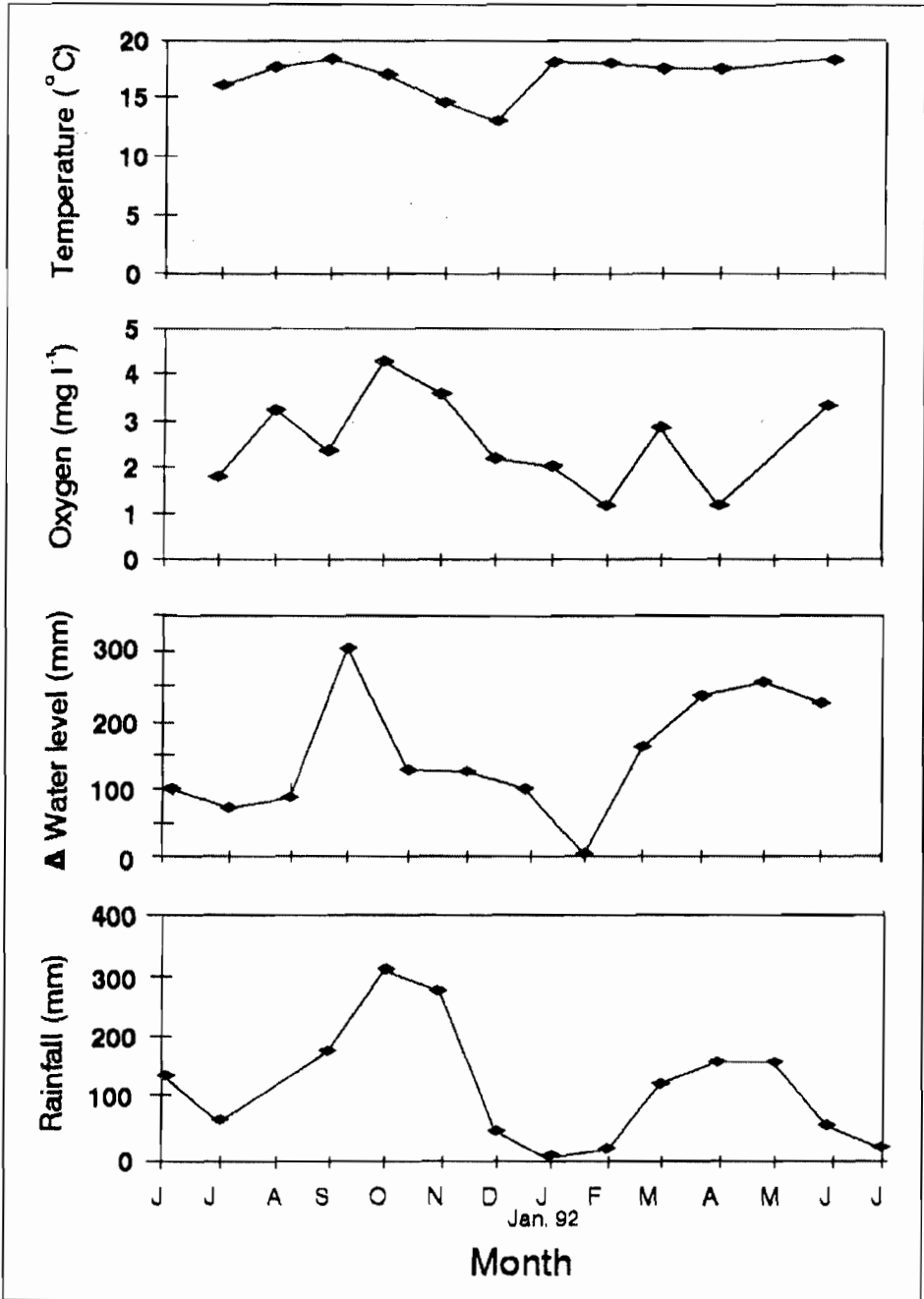
Figure 1: Monthly values a) water temperature (°C), b) dissolved oxygen concentration (mg l -1 ), c) water level change (mm), and d) rainfall (mm) for the Inlet Stream East of the Rwembaita Swamp in Kibale National Park, Uganda
