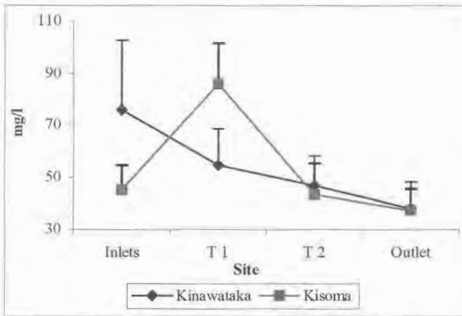
Figure 5. Comparison of Total Nitrogen (TN) in Kinawataka and Kisoma wetlands
